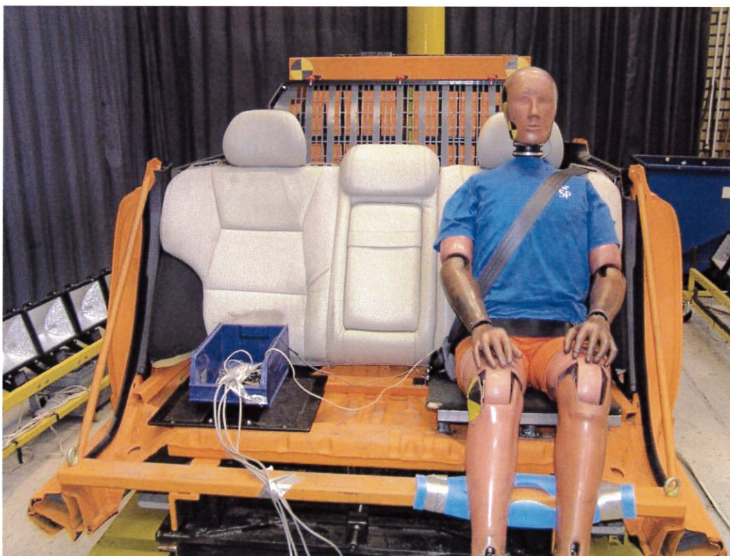
02 – Before test, rear impact
