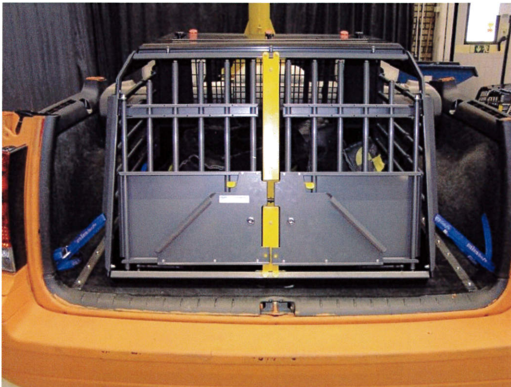
Figure 1 Test setup Frontal impact crash test
